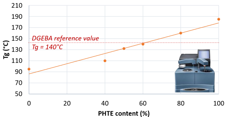
T g as function of PHTE/DGEVA ratio
